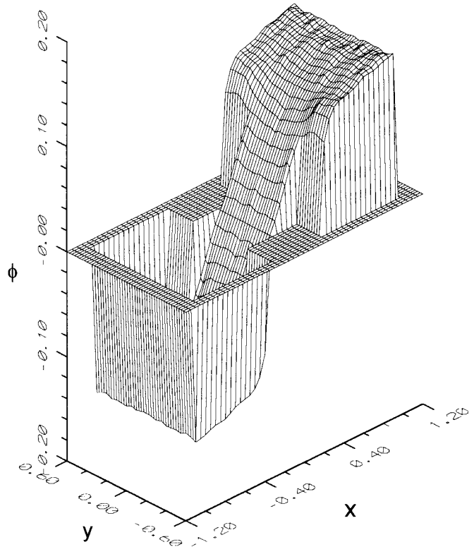
Fig. 3. Double-ridge waveguide. TE fundamental mode. ( a = 2b = 2 , W/a = 0.3, S/b = 0.5 .)
