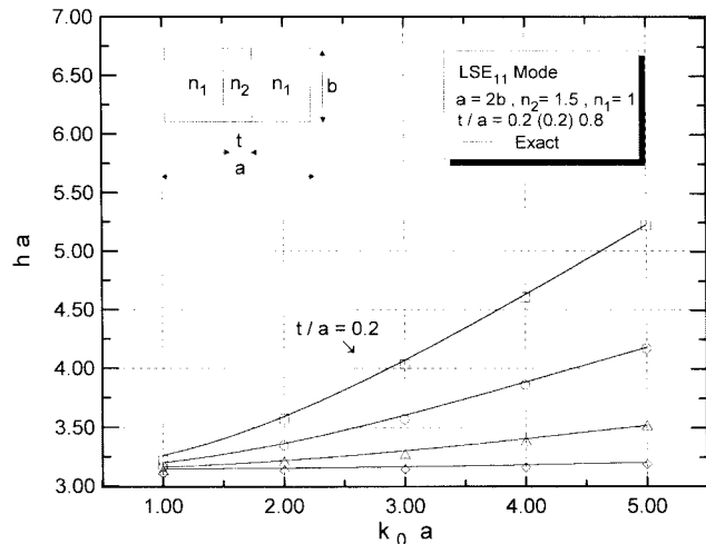
Fig. 4. Dielectric loaded rectangular waveguide. LSE_{11} mode dispersion diagram ( h = [k_0^2 n_1^2 - (\pi/b)^2]^{1/2} ) at various values of dielectric slab thickness. Continuous line: exact solution; markers: GDK method.
