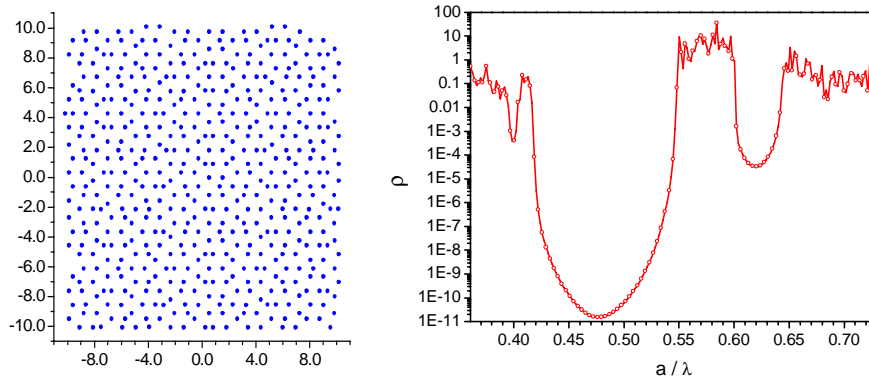
Fig. 1. Left: A Penrose photonic quasicrystal made of 530 dielectric rods placed at the vertices of the rhombus tiles. Right: LDOS computed at x = 0, y = 0 . Distances are normalized with respect to a in all figs.
